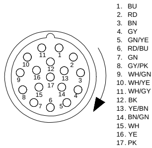
FEMALE END VIEW
